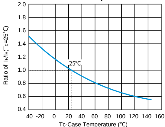
Fig.3 Normalized DC Holding Current versus Case Temperature
